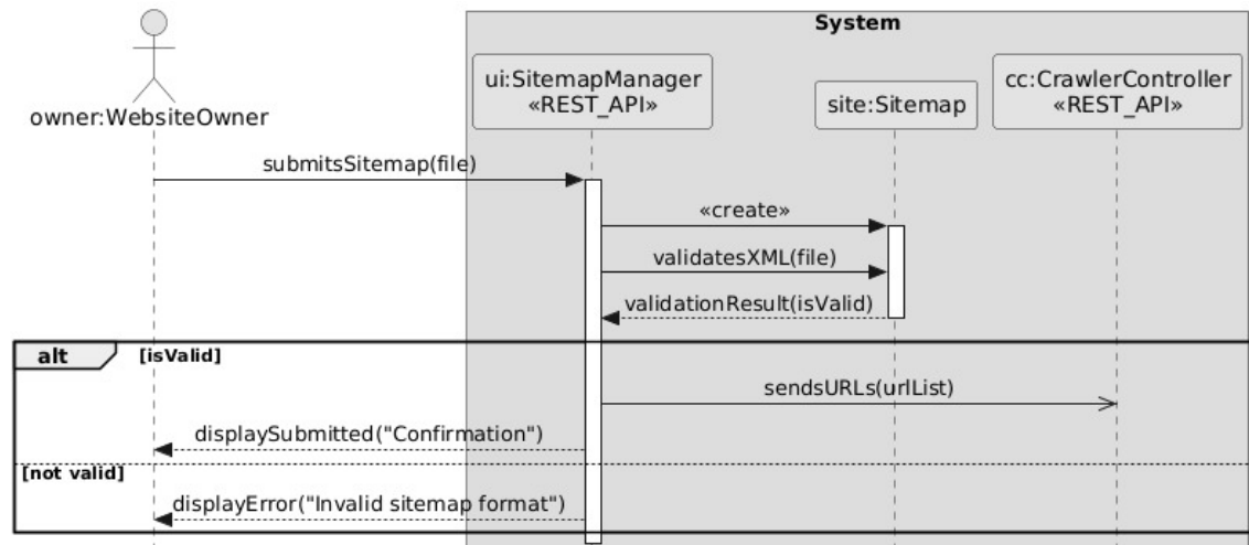
Figure 3: Sequence Diagram: Sitemap Submission via REST.
